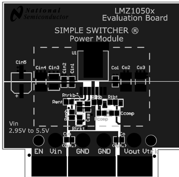
FIGURE 6. Top Copper
