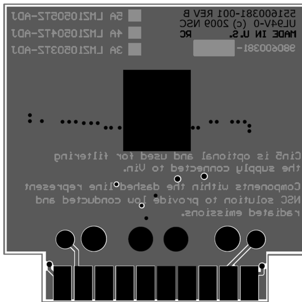
FIGURE 9. Bottom Copper
